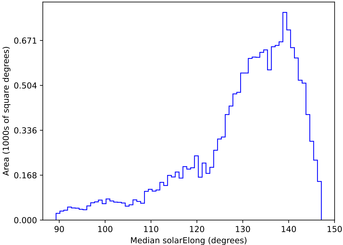
too_ignore_10_1v3.4_10yrs WFD y band: Median solarElong
