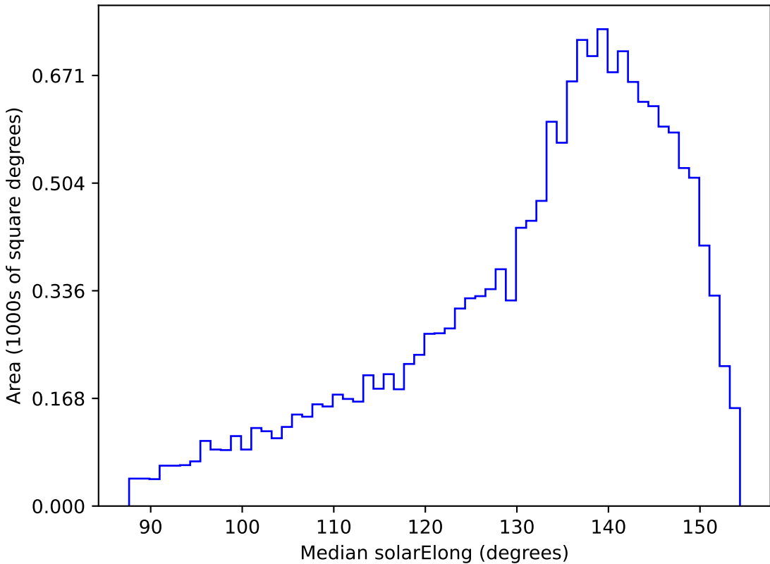
too_ignore_10_1v3.4_10yrs WFD u band: Median solarElong
