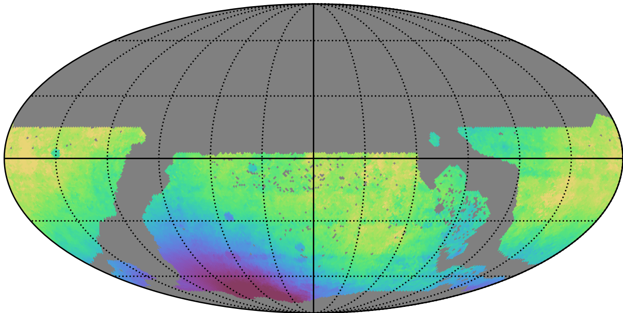
too_ignore_10_1v3.4_10yrs WFD r band: Median solarElong
