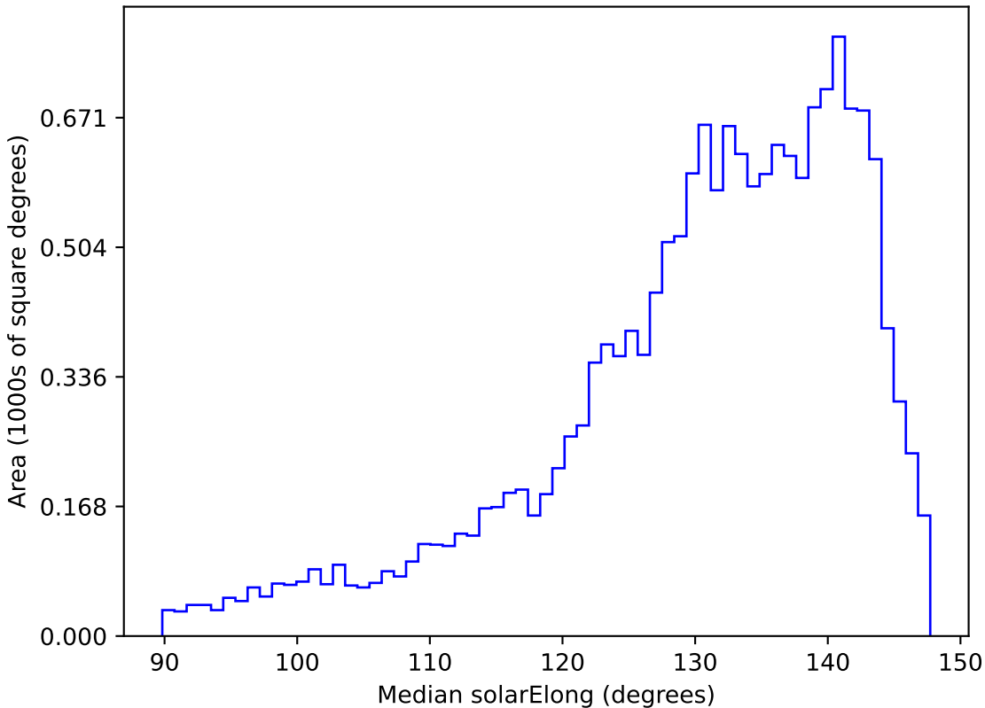
too_ignore_10_1v3.4_10yrs WFD r band: Median solarElong
