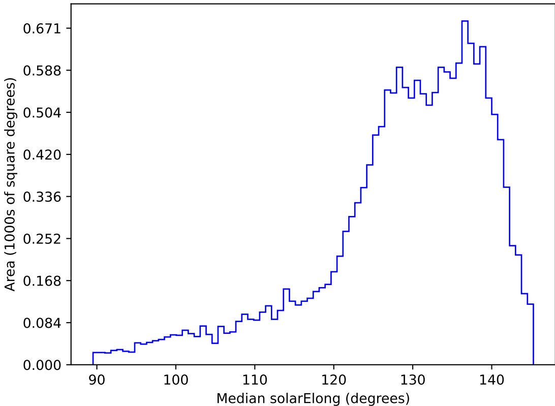
too_ignore_10_1v3.4_10yrs WFD i band: Median solarElong
