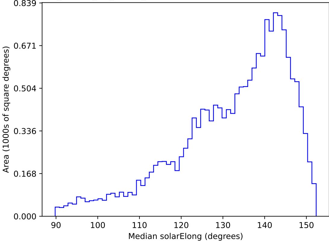
too_ignore_10_1v3.4_10yrs WFD g band: Median solarElong
