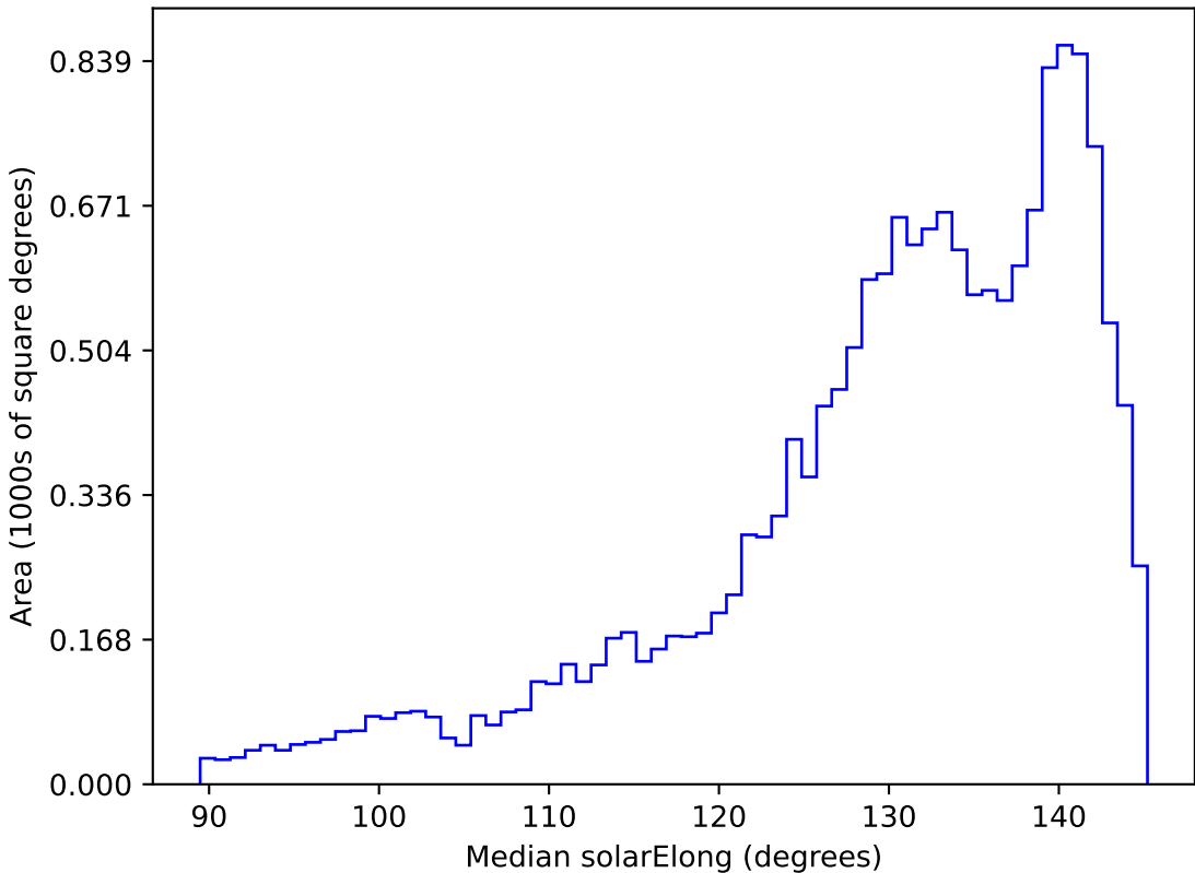
too_ignore_10_1v3.4_10yrs WFD all bands: Median solarElong
