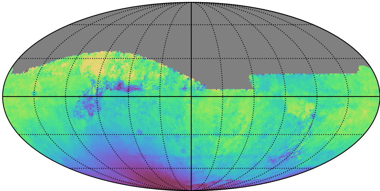
too_ignore_10_1v3.4_10yrs All sky z band: Median solarElong
