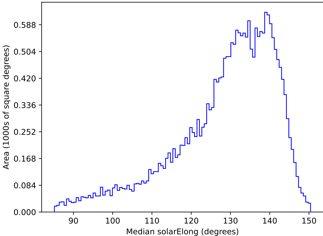
too_ignore_10_1v3.4_10yrs All sky y band: Median solarElong
