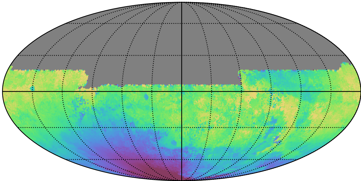
too_ignore_10_1v3.4_10yrs All sky u band: Median solarElong
