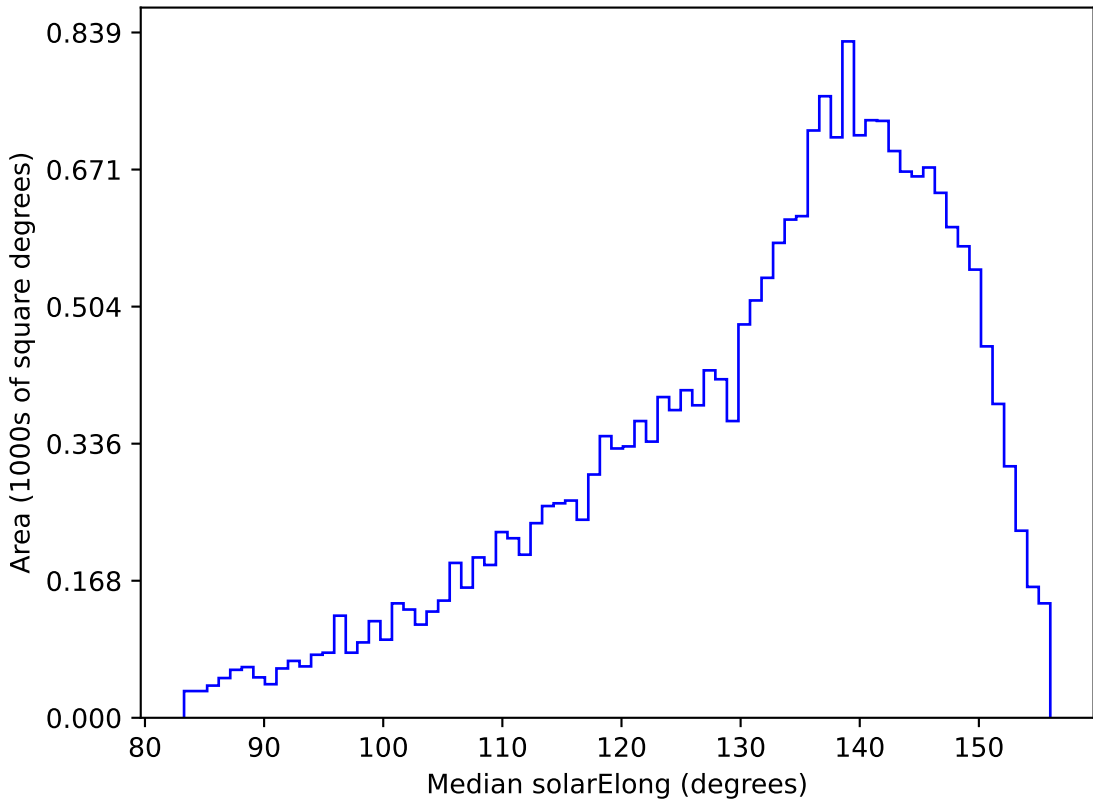
too_ignore_10_1v3.4_10yrs All sky u band: Median solarElong
