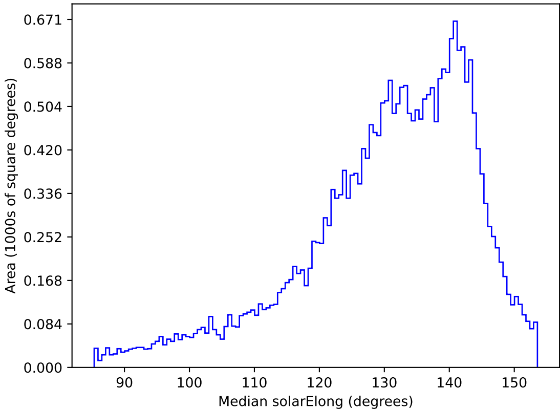
too_ignore_10_1v3.4_10yrs All sky r band: Median solarElong
