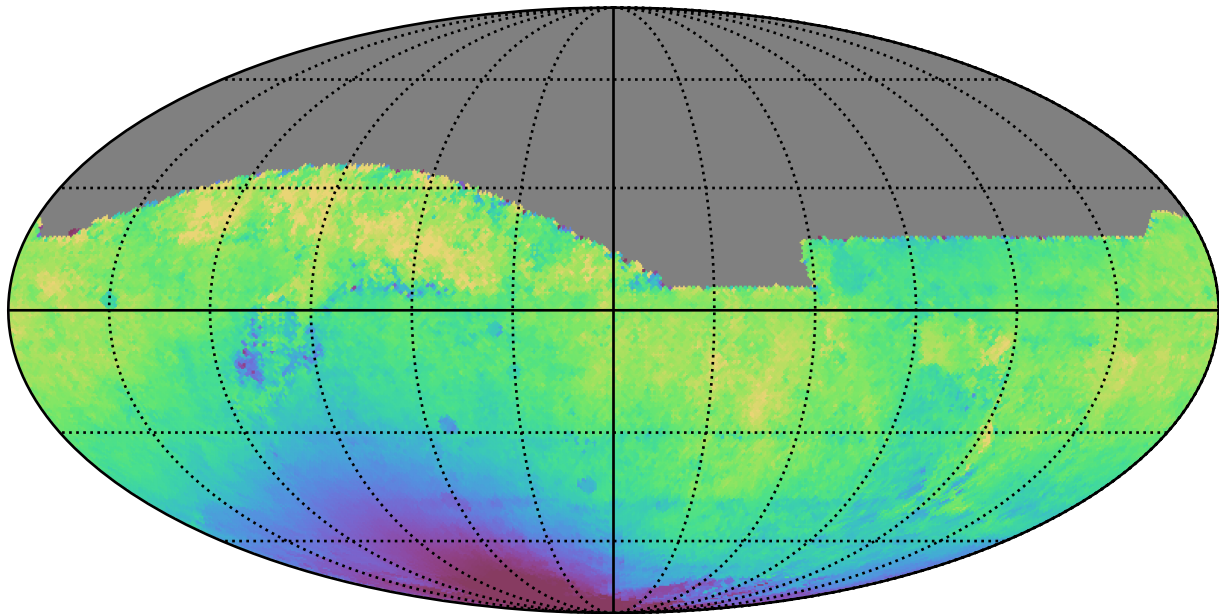
too_ignore_10_1v3.4_10yrs All sky i band: Median solarElong
