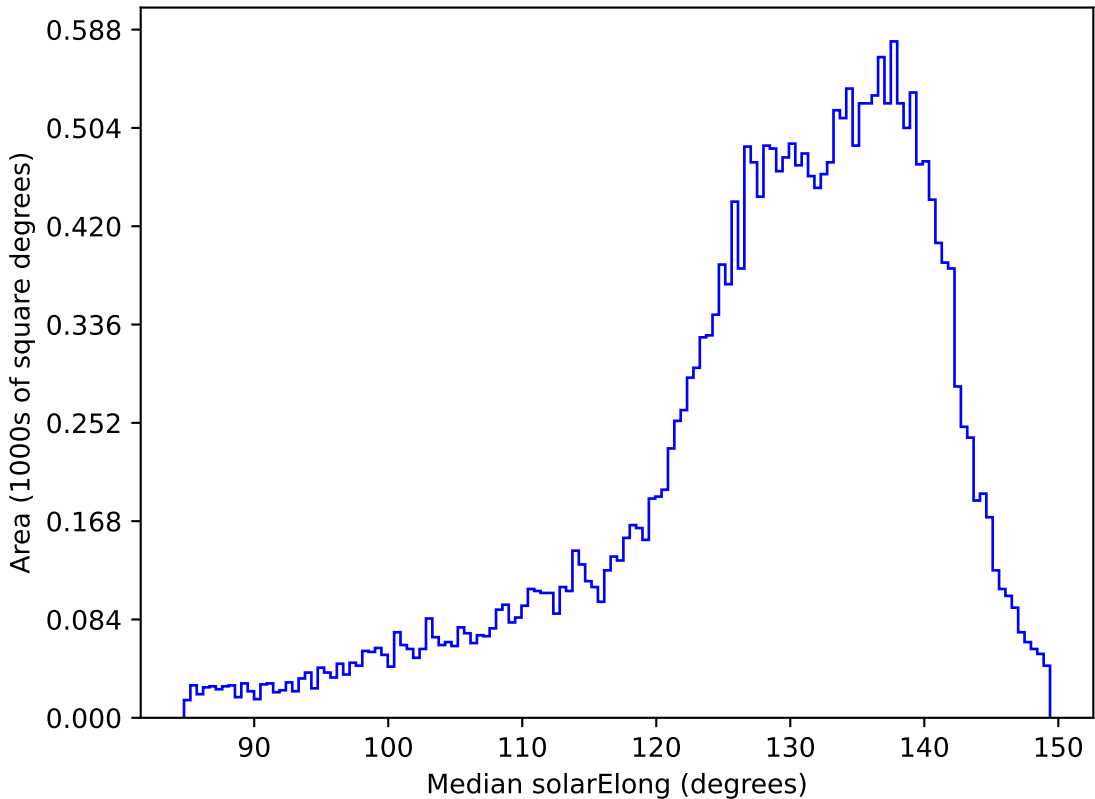
too_ignore_10_1v3.4_10yrs All sky i band: Median solarElong
