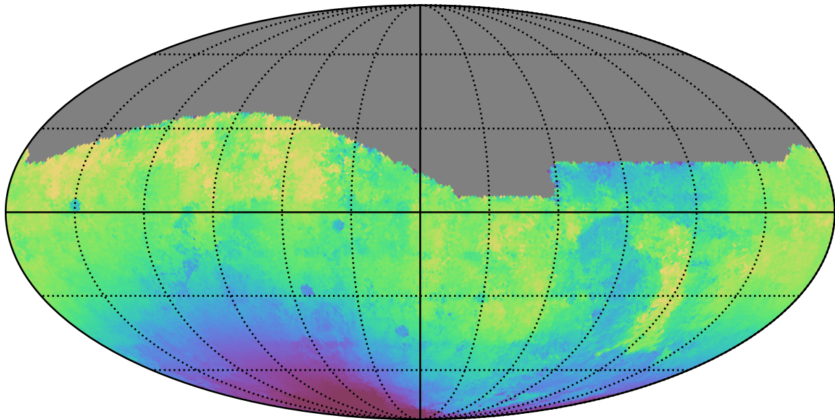
too_ignore_10_1v3.4_10yrs All sky g band: Median solarElong
