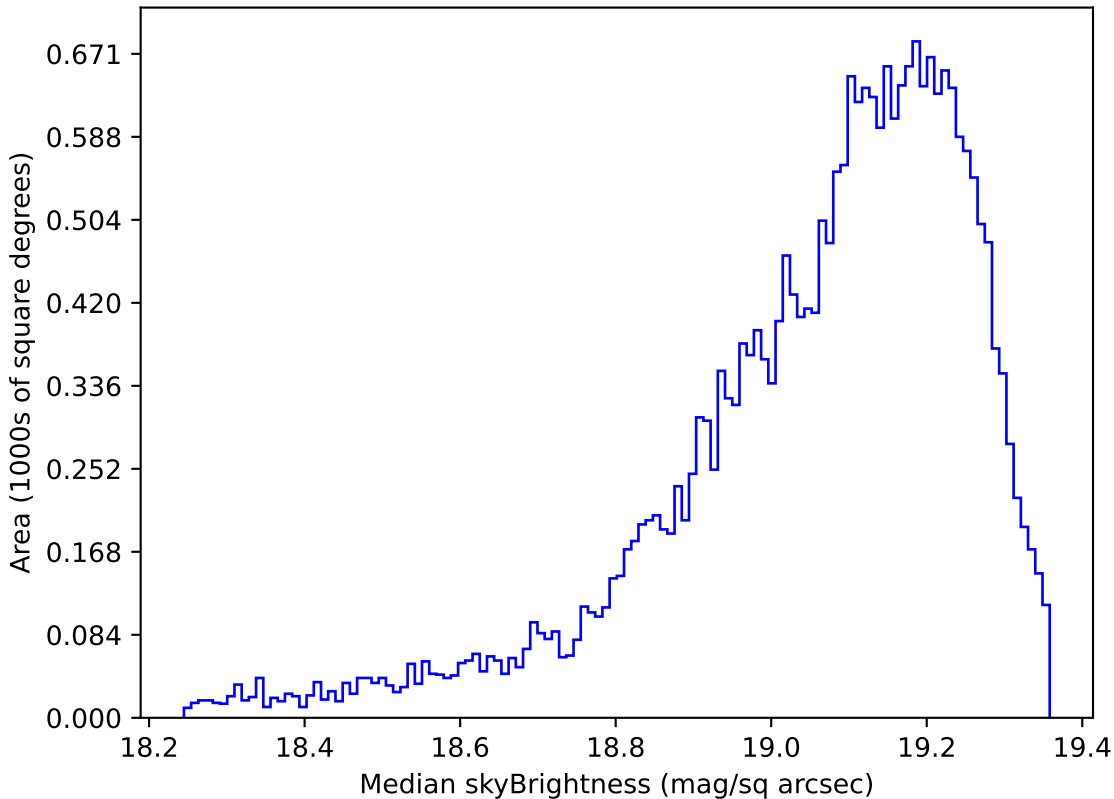
too_ignore_10_1v3.4_10yrs Yr 1 z band: Median skyBrightness
