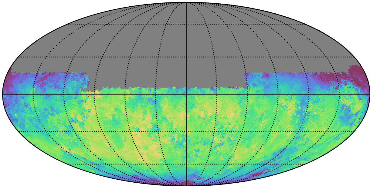
too_ignore_10_1v3.4_10yrs Yr 1 y band: Median skyBrightness
