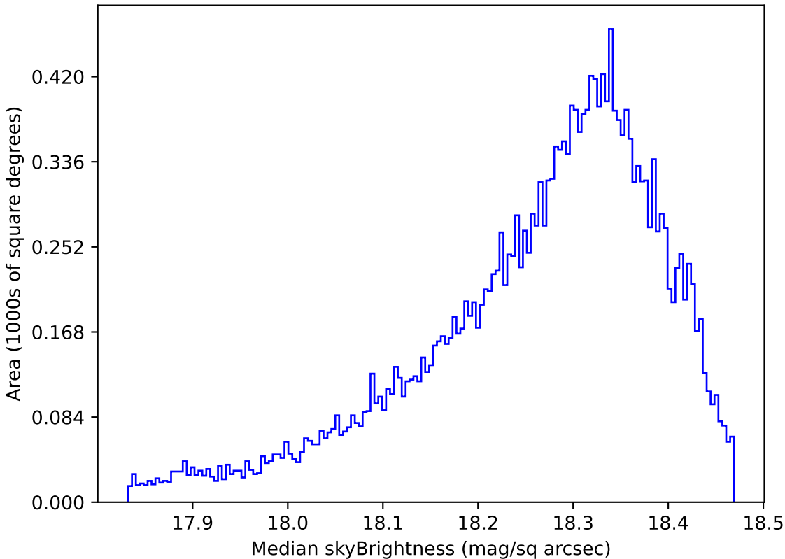
too_ignore_10_1v3.4_10yrs Yr 1 y band: Median skyBrightness
