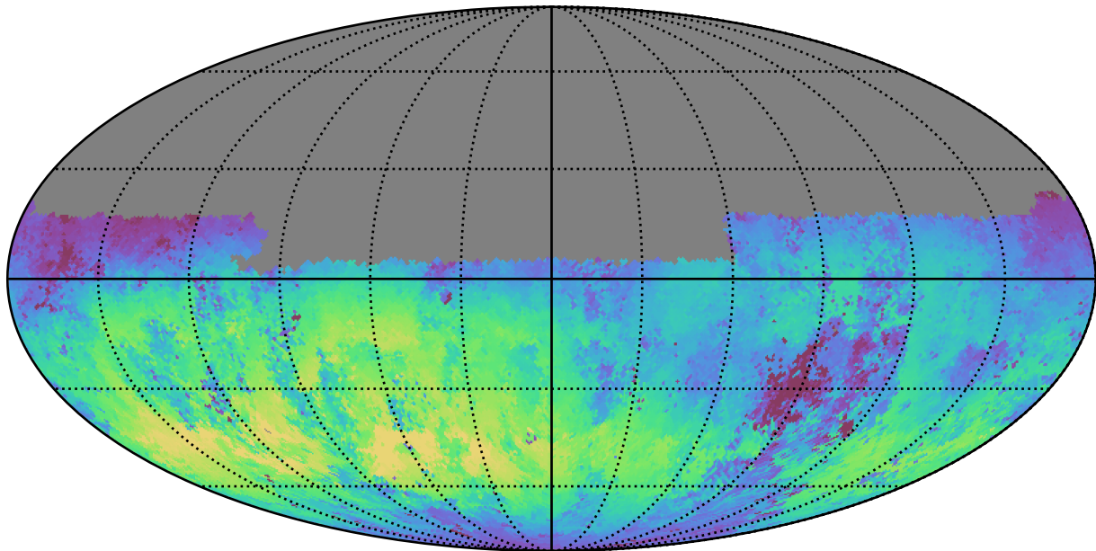
too_ignore_10_1v3.4_10yrs Yr 1 u band: Median skyBrightness
