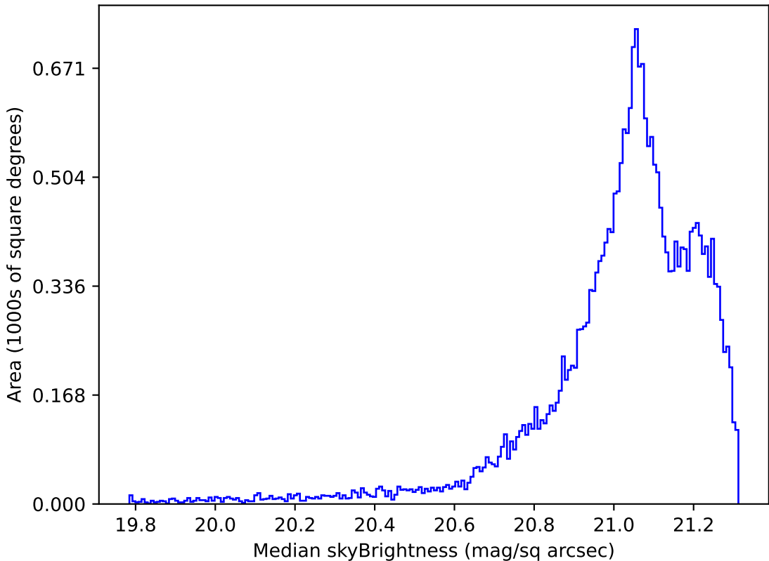
too_ignore_10_1v3.4_10yrs Yr 1 r band: Median skyBrightness
