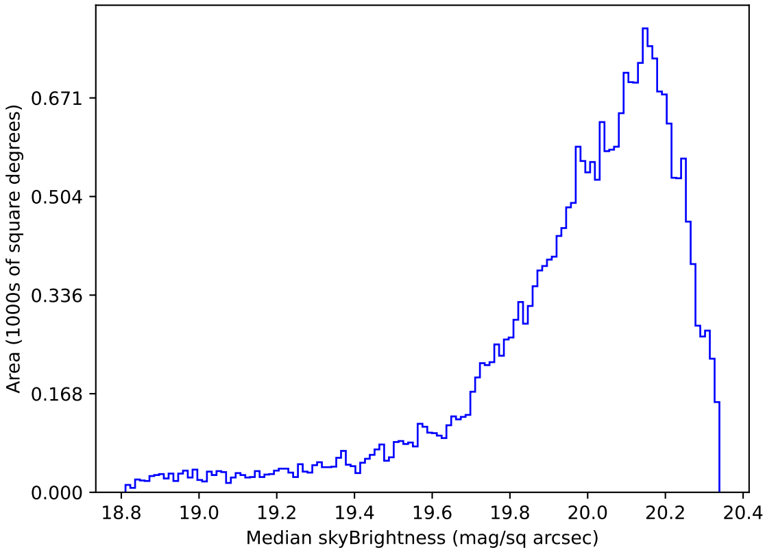
too_ignore_10_1v3.4_10yrs Yr 1 i band: Median skyBrightness
