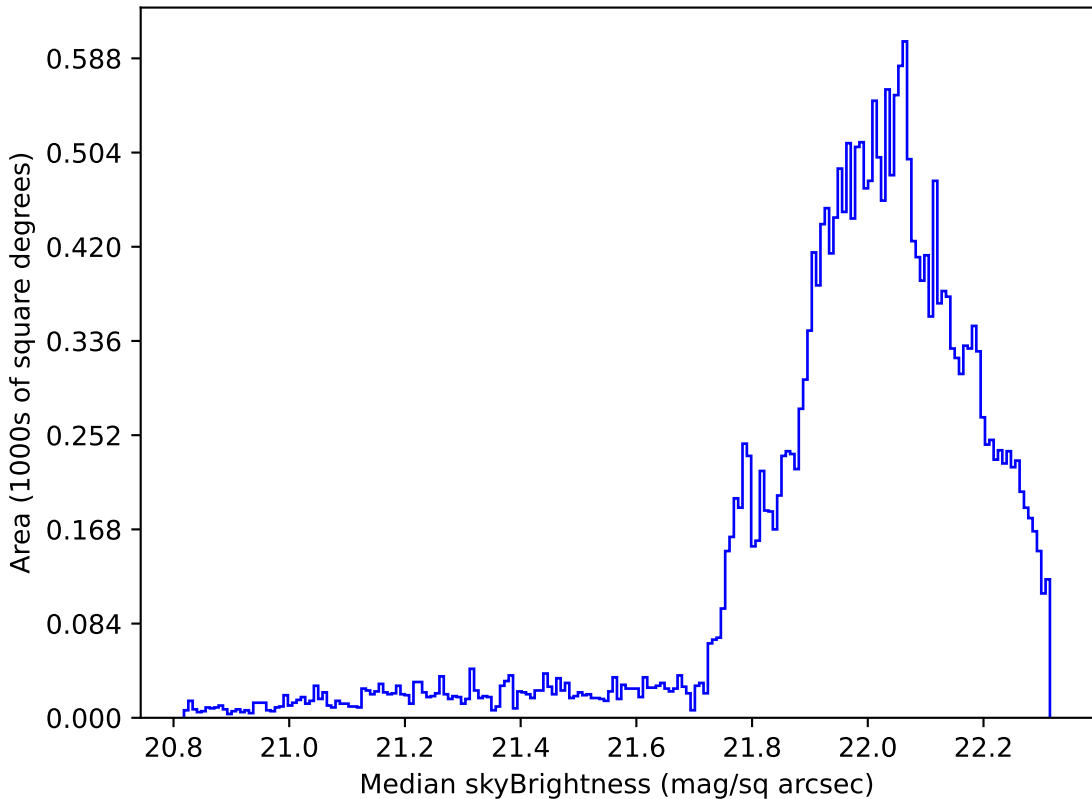
too_ignore_10_1v3.4_10yrs Yr 1 g band: Median skyBrightness
