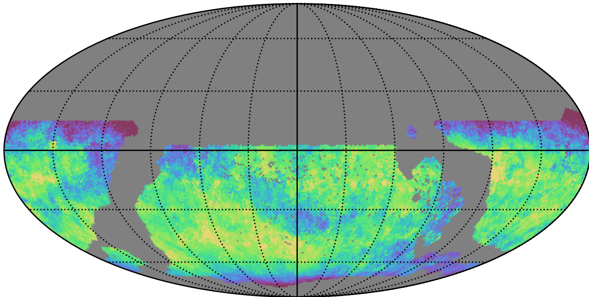
too_ignore_10_1v3.4_10yrs WFD z band: Median skyBrightness
