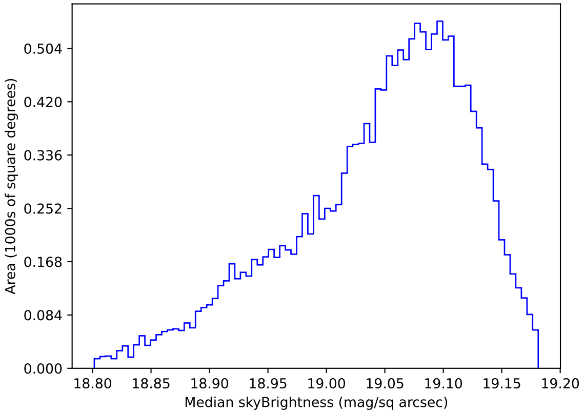
too_ignore_10_1v3.4_10yrs WFD z band: Median skyBrightness
