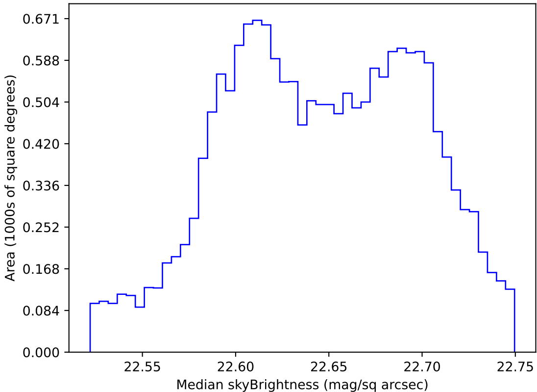
too_ignore_10_1v3.4_10yrs WFD u band: Median skyBrightness
