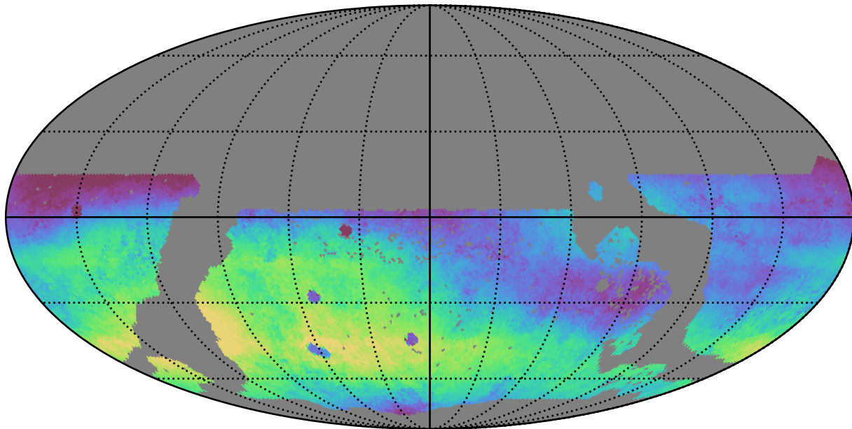
too_ignore_10_1v3.4_10yrs WFD r band: Median skyBrightness
