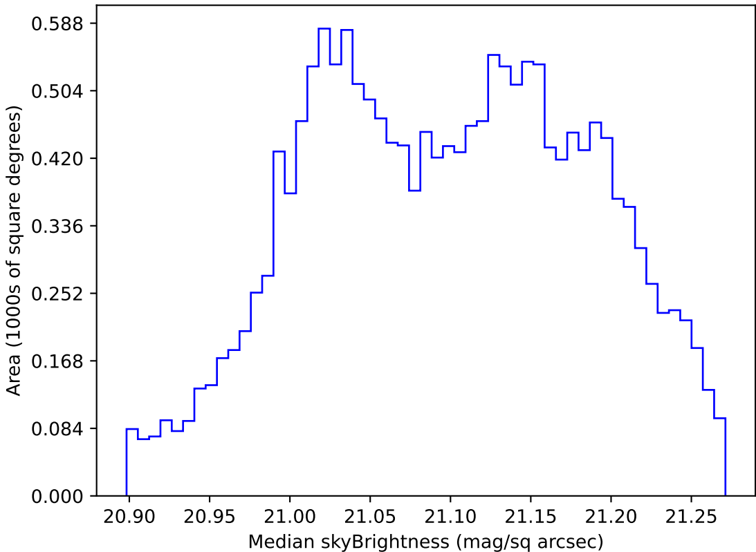
too_ignore_10_1v3.4_10yrs WFD r band: Median skyBrightness
