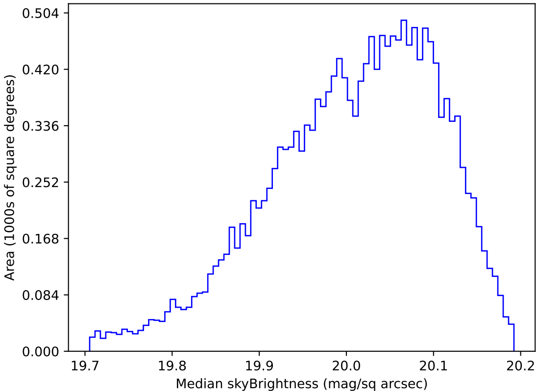
too_ignore_10_1v3.4_10yrs WFD i band: Median skyBrightness
