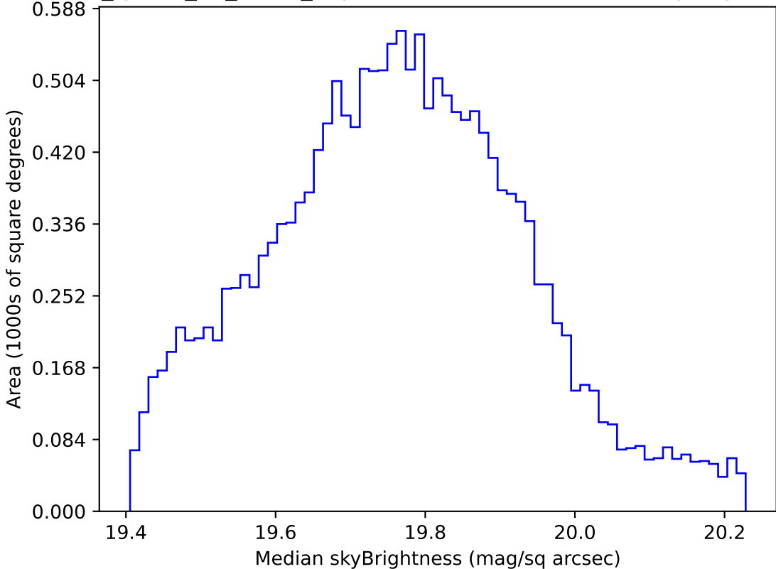
too_ignore_10_1v3.4_10yrs WFD all bands: Median skyBrightness
