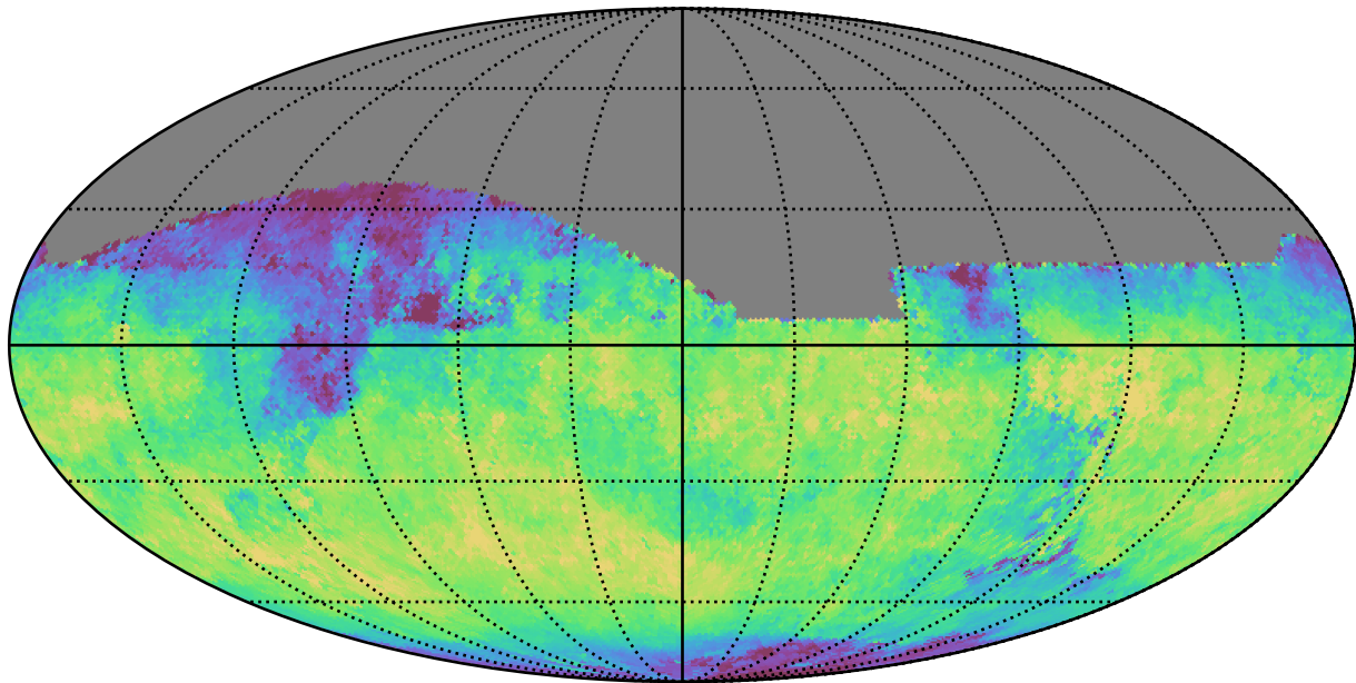
too_ignore_10_1v3.4_10yrs All sky z band: Median skyBrightness
