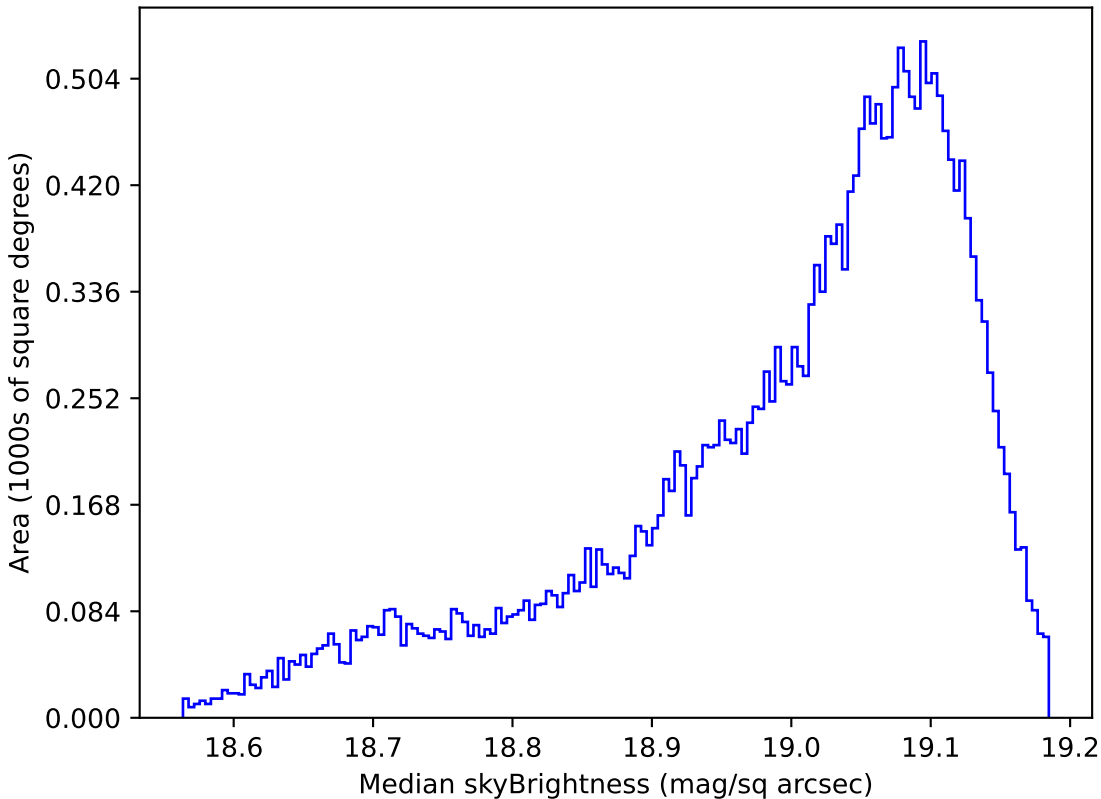
too_ignore_10_1v3.4_10yrs All sky z band: Median skyBrightness
