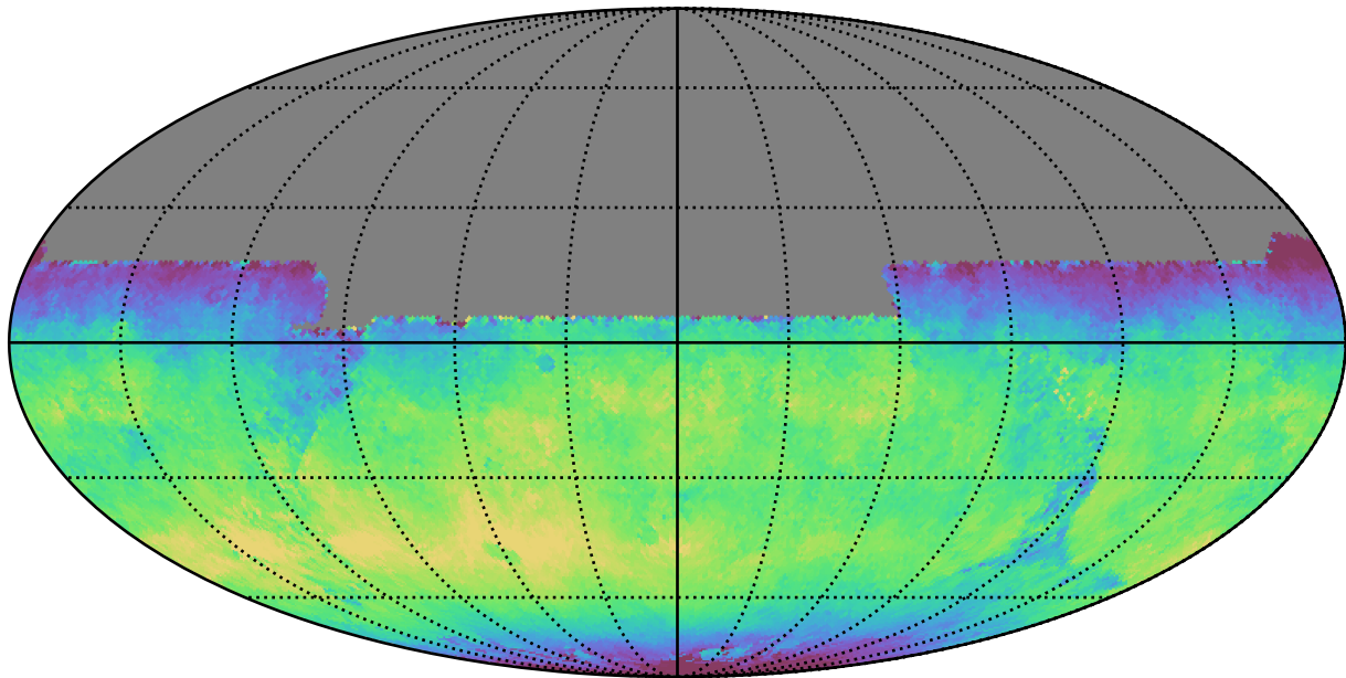
too_ignore_10_1v3.4_10yrs All sky y band: Median skyBrightness
