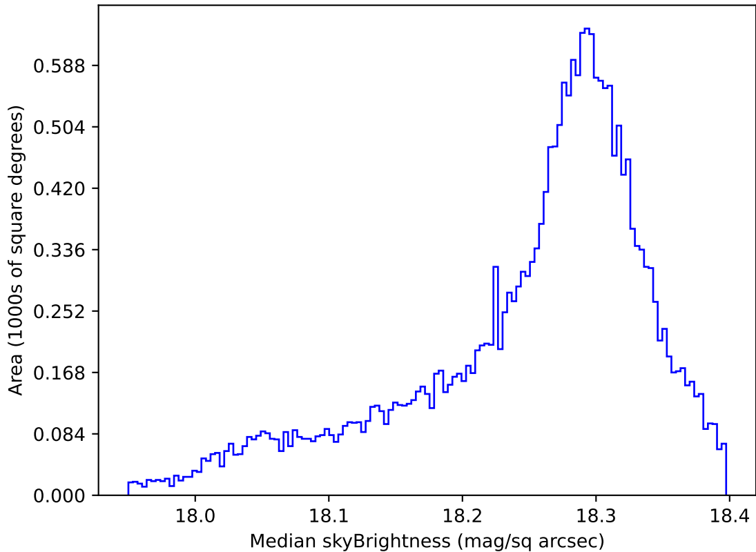
too_ignore_10_1v3.4_10yrs All sky y band: Median skyBrightness
