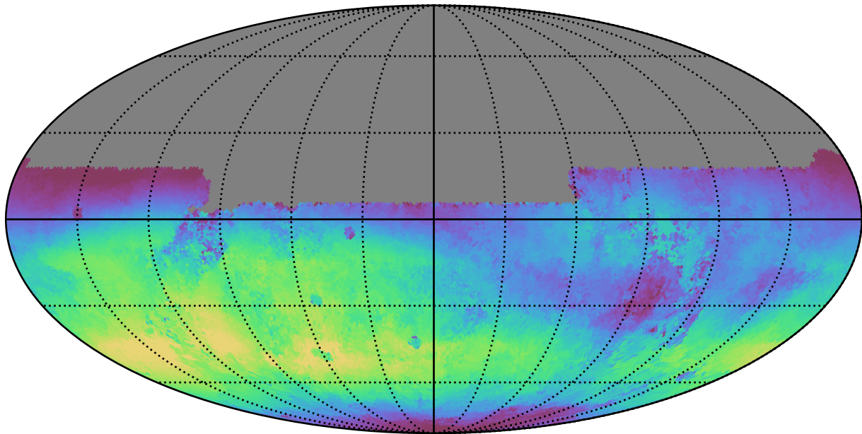
too_ignore_10_1v3.4_10yrs All sky u band: Median skyBrightness
