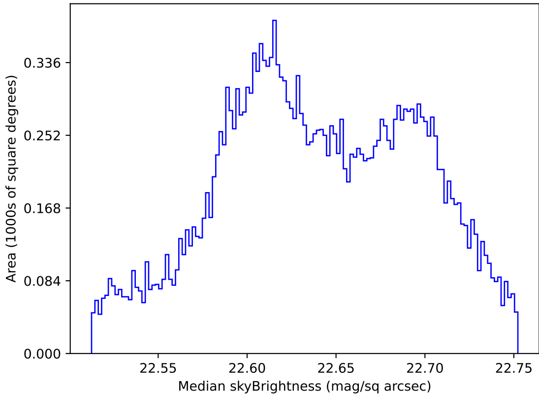
too_ignore_10_1v3.4_10yrs All sky u band: Median skyBrightness
