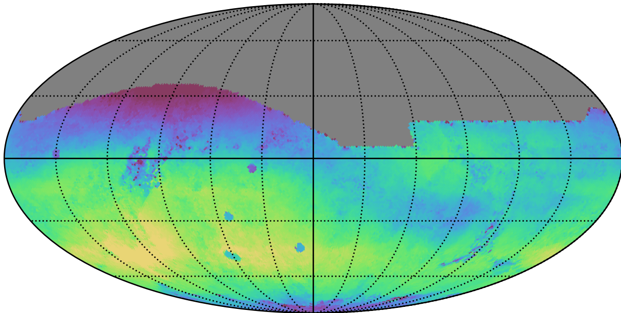
too_ignore_10_1v3.4_10yrs All sky r band: Median skyBrightness
