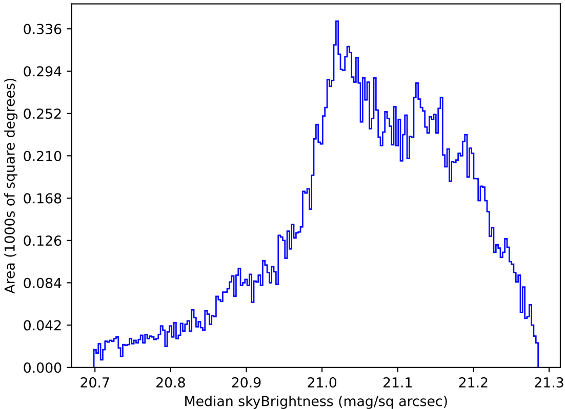
too_ignore_10_1v3.4_10yrs All sky r band: Median skyBrightness
