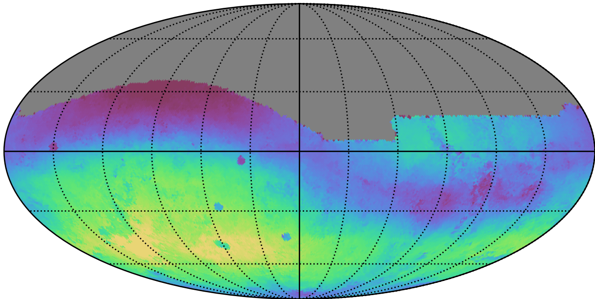
too_ignore_10_1v3.4_10yrs All sky g band: Median skyBrightness
