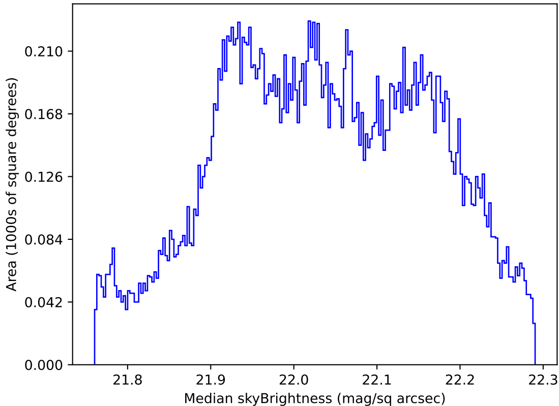
too_ignore_10_1v3.4_10yrs All sky g band: Median skyBrightness
