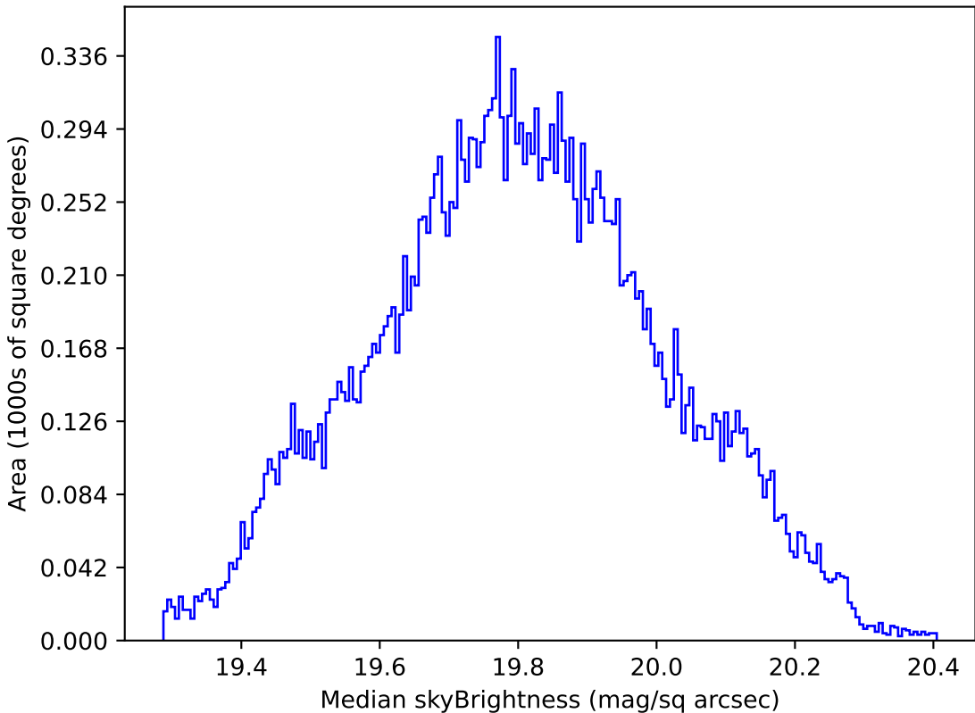
too_ignore_10_1v3.4_10yrs All sky all bands: Median skyBrightness
