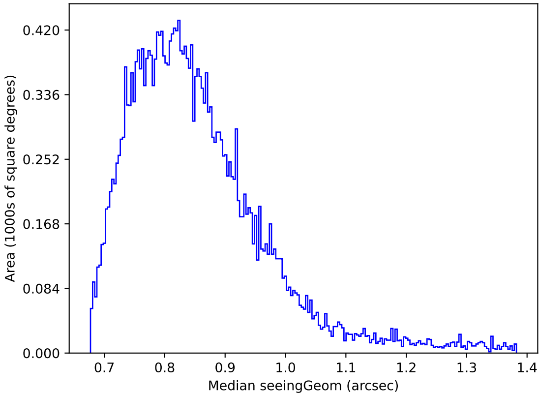
too_ignore_10_1v3.4_10yrs Yr 1 z band: Median seeingGeom
