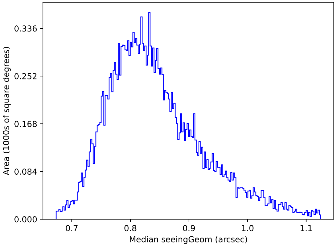
too_ignore_10_1v3.4_10yrs Yr 1 y band: Median seeingGeom
