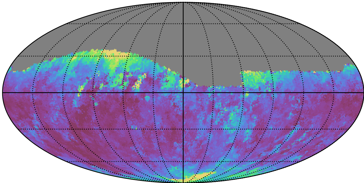
too_ignore_10_1v3.4_10yrs Yr 1 r band: Median seeingGeom
