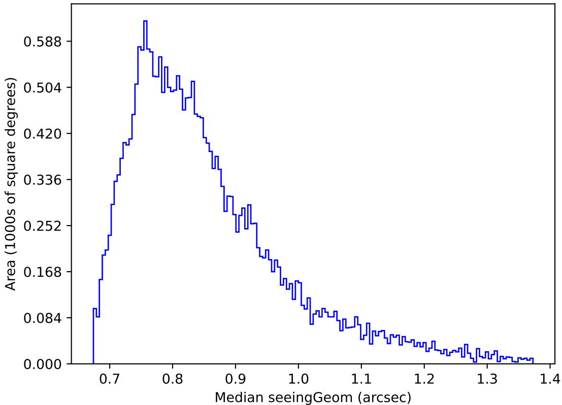
too_ignore_10_1v3.4_10yrs Yr 1 r band: Median seeingGeom
