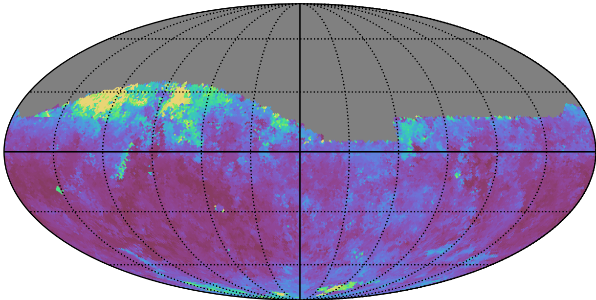
too_ignore_10_1v3.4_10yrs Yr 1 i band: Median seeingGeom
