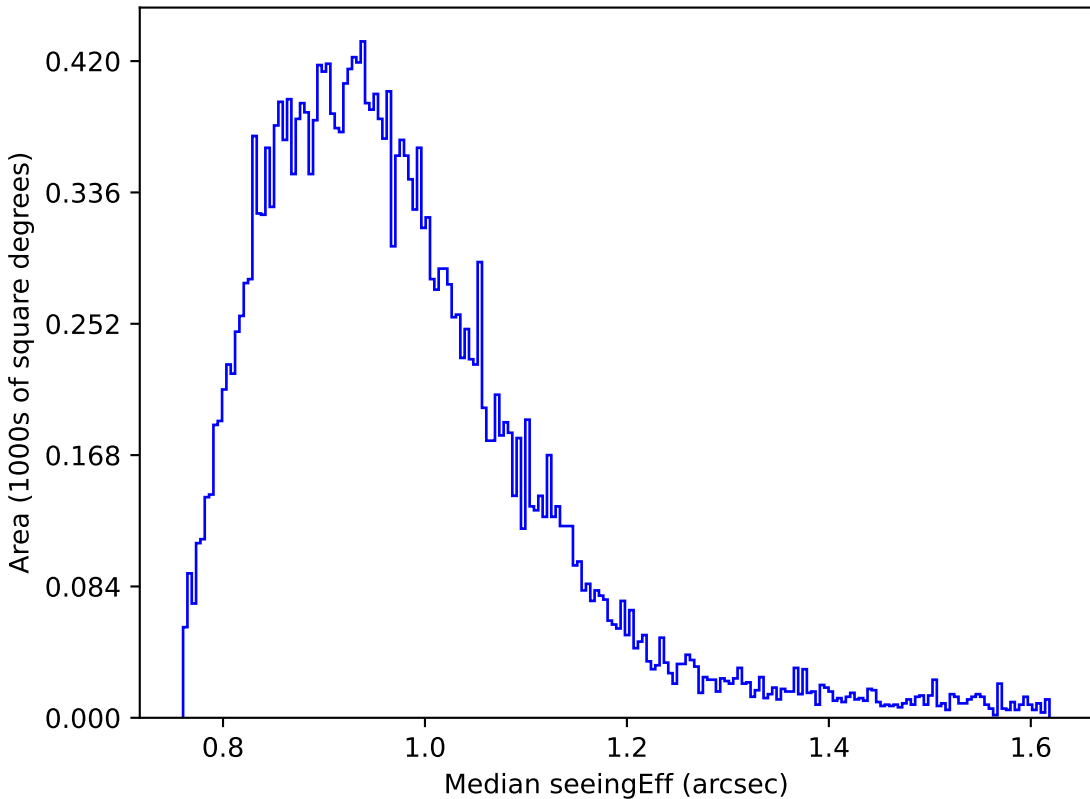
too_ignore_10_1v3.4_10yrs Yr 1 z band: Median seeingEff
