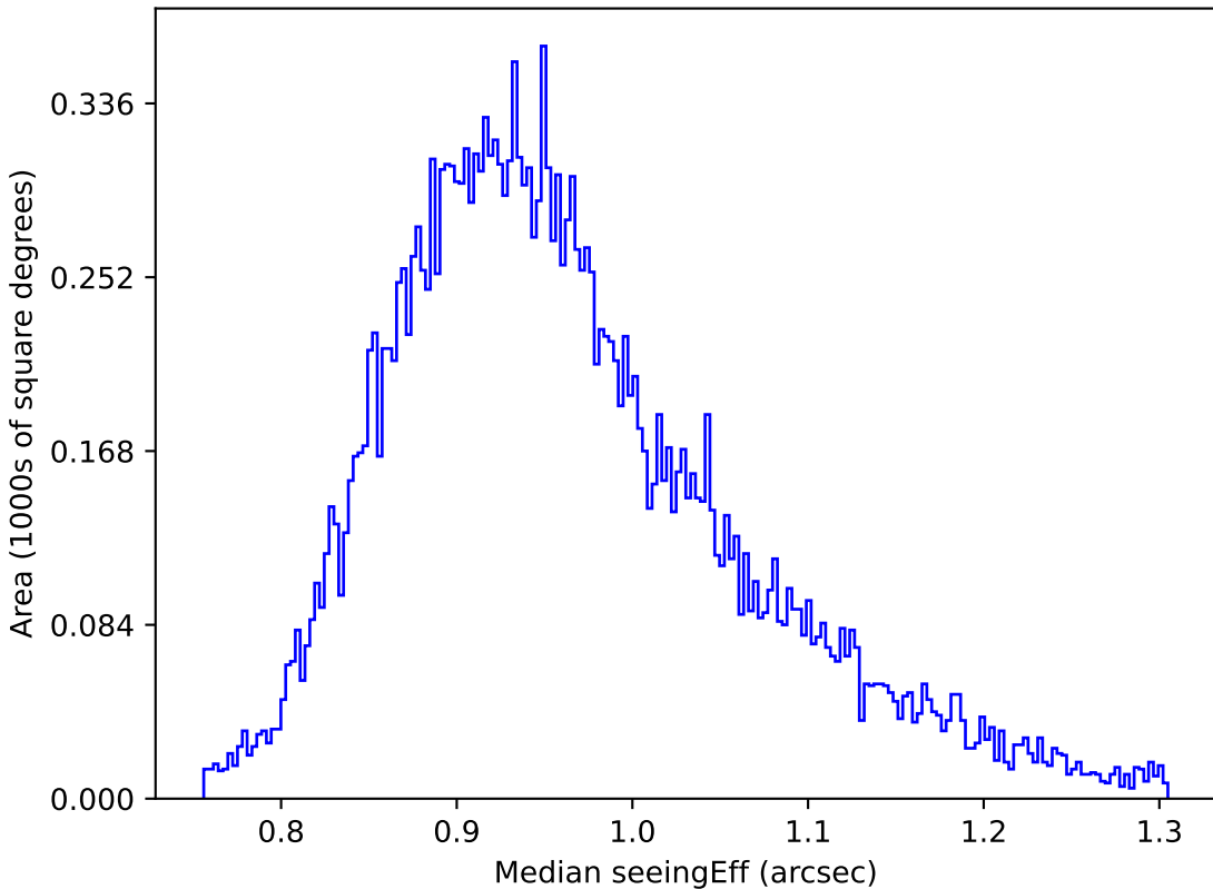
too_ignore_10_1v3.4_10yrs Yr 1 y band: Median seeingEff
