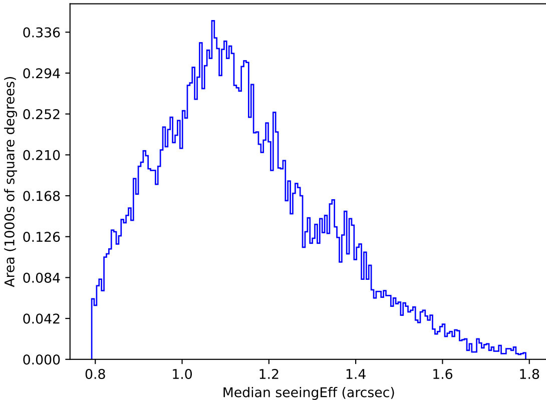
too_ignore_10_1v3.4_10yrs Yr 1 u band: Median seeingEff
