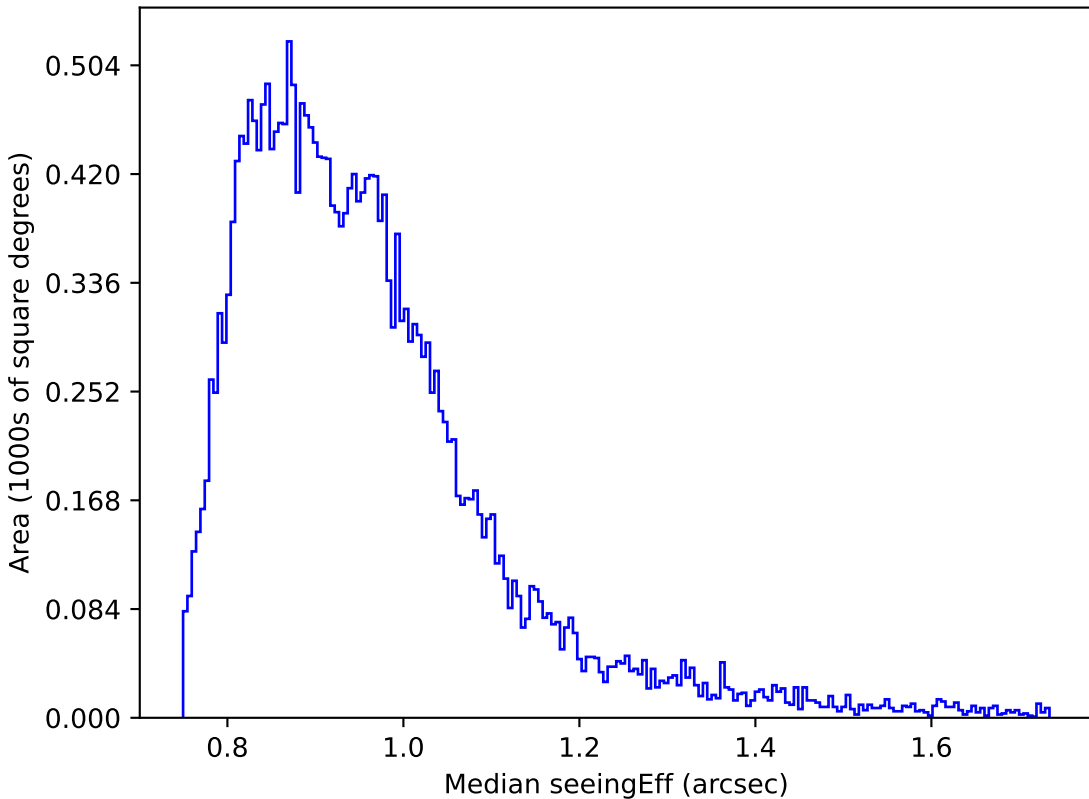
too_ignore_10_1v3.4_10yrs Yr 1 i band: Median seeingEff
