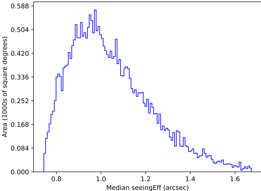
too_ignore_10_1v3.4_10yrs Yr 1 g band: Median seeingEff
